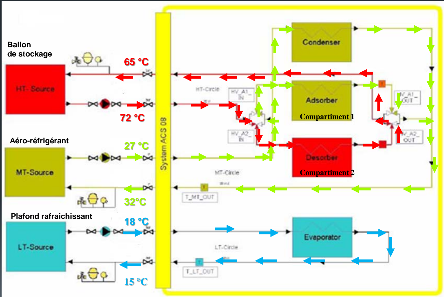
Compartment 1 = adsorbeur compartment 2 = désorbeur
